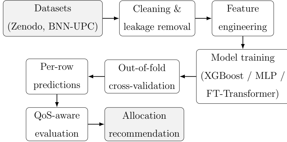
Figure 4.1: End-to-end experimental workflow, from raw datasets to the allocation recommendation. Leakage columns are removed before feature engineering; models are compared under an identical out-of-fold cross-validation protocol; and the resulting per-row predictions feed both the QoS-aware evaluation and the Layer 3 recommender.
